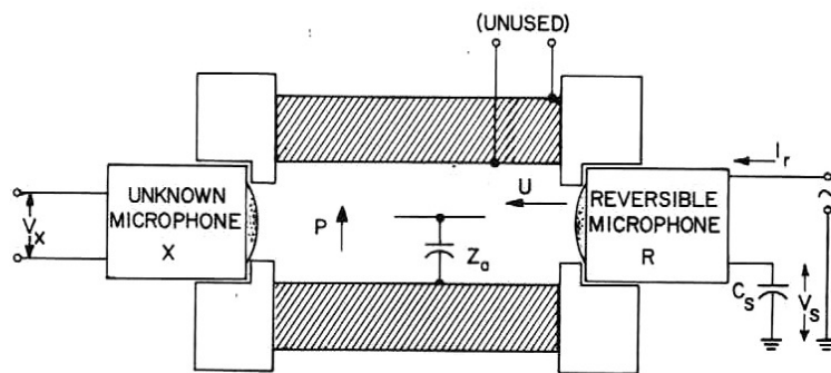
Figure 3-6. Conditions for determining the product of microphone sensitivities.
