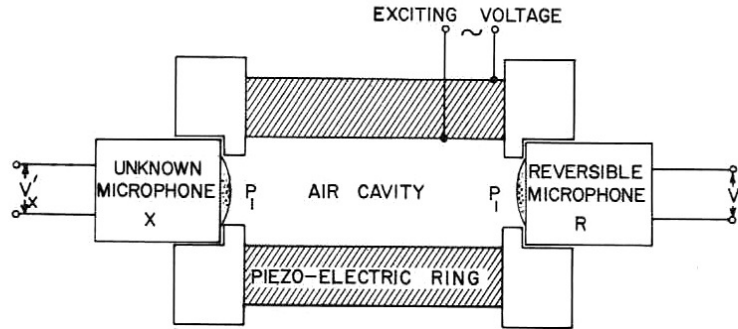
Figure 3-5. Conditions for determining the ratio of microphone sensitivities.
