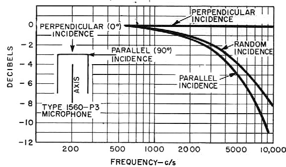
Figure 2-5. Corrections to be added to free-field perpendicular-incidence response for random- and parallel-incidence responses of Types 1560-P1 and -P3 Microphones and Type 1560-P4 Microphone Assembly.
