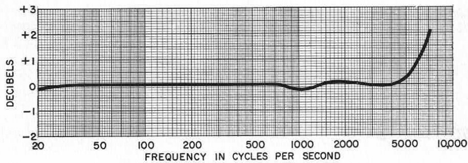
Figure 2-7. Average deviation of the calibration by the Type 1559-B Microphone Reciprocity Calibrator from the true random incidence for the W E 640AA Microphone.
