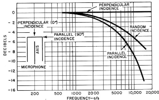
Figure 2-4. Corrections to be added to free-field perpendicular-incidence response for random- and parallel-incidence responses of W E 640AA and Type 1560-P5 Microphones and Type 1560-P6 Microphone Assembly.
