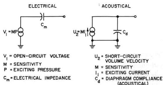
Figure 3-4. Equivalent circuits of a ceramic microphone.
