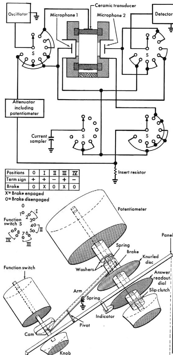
Figure 3-8. The analog-computer mechanism.
