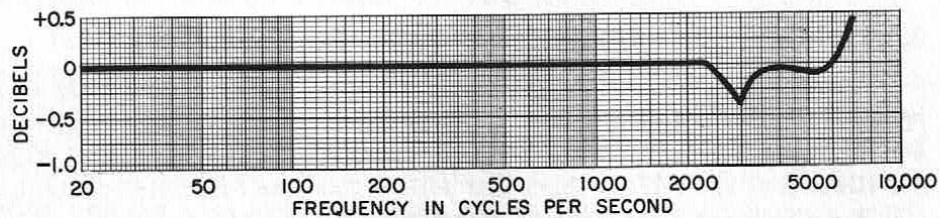
Figure 2-8. Average deviation of calibration by the Type 1559-B Microphone Reciprocity Calibrator from the true random incidence for the General Radio Types 1560-P1 and -P3 Microphones and Type 1560-P4 Microphone Assembly.
