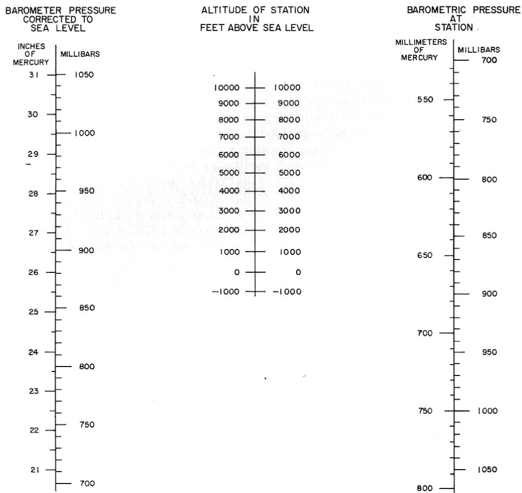
Figure 2-1. Nomograph for applying altitude correction to barometric pressure. Place straight-edge across proper points on center and left-hand scales and read actual pressure on right-hand scale. See Appendix 2 for altitudes above sea level for many cities in the U.S. and Canada.
