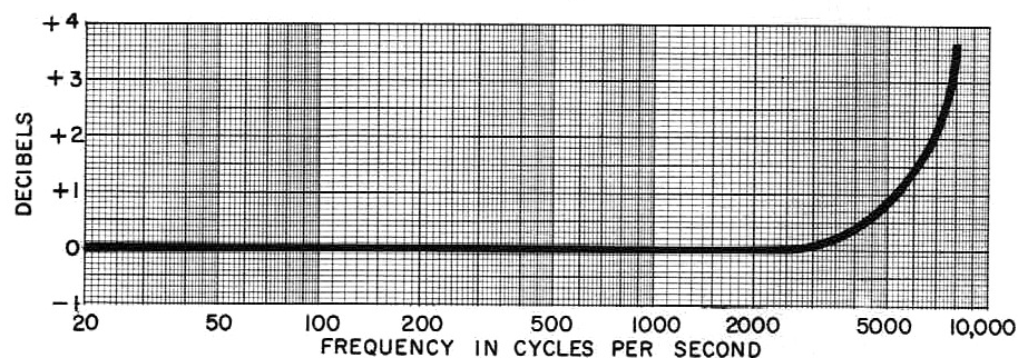
Figure 2-6. Average deviation of the calibration by the Type 1559-B Microphone Reciprocity Calibrator from the true random incidence for the General Radio Type 1560-P5 Microphone and Type 1560-P6 Microphone Assembly.
