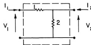
Figure 3-1. The Principle of Reciprocity applied to a two-port, four-terminal network.
