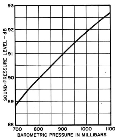
Figure 2-3. Sound-level calibration output versus atmospheric pressure.
