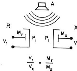
Figure 3-3. Relationships of three transducers in reciprocity calibration.
