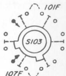
Figure 5-9. Switching diagram of Type 1806-A Electronic Voltmeter.
